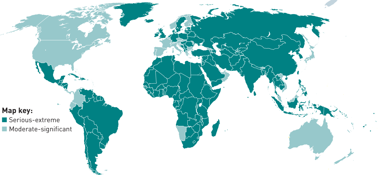
Global exposure to climate change
